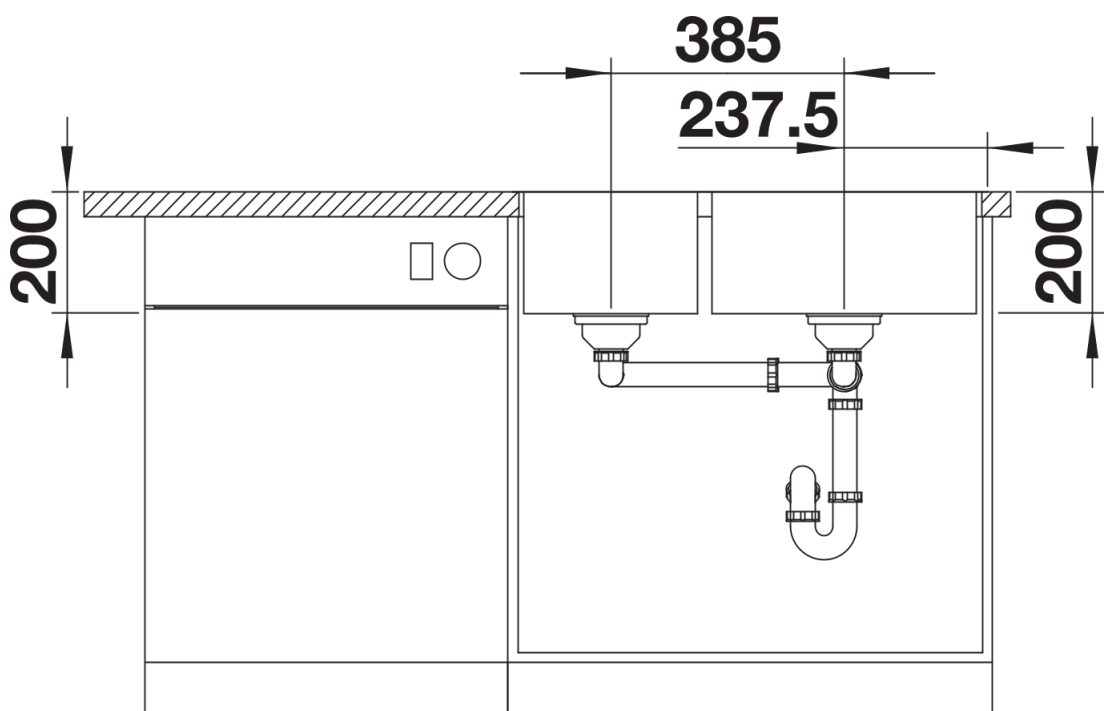
Front view
