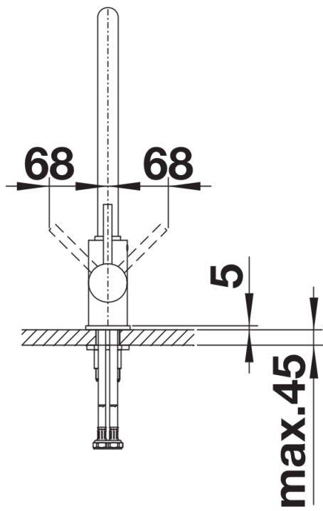
Side view hand gear 2D
