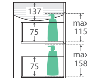
SIDE VIEW: RECESS & DRAWER STORAGE
