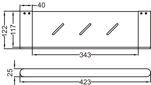
METAL SHOWER SHELF NR9087aCH / NR9087aMB / NR9087aBN NR9087aGM / NR9087aBG
