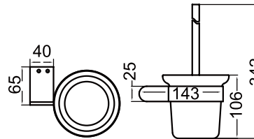
TOILET BRUSH HOLDER NR9088CH / NR9088MB / NR9088BN NR9088GM / NR9088BG
