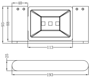
SOAP DISH HOLDER NR9081CH / NR9081MB / NR9081BN NR9081GM / NR9081BG
