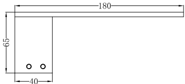
TOILET ROLL HOLDER WITH PHONE HOLDER NR9086aCH / NR9086aMB / NR9086aBN NR9086aGM / NR9086aBG
