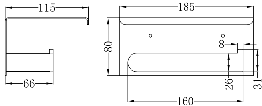
HAND TOWEL RAIL NR9080CH / NR9080MB / NR9080BN NR9080GM / NR9080BG
