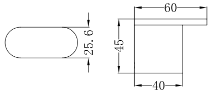
TOILET ROLL HOLDER NR9086CH / NR9086MB / NR9086BN NR9086GM / NR9086BG
